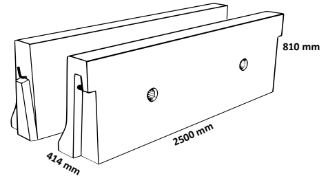
810 CPB Pier Barrier
